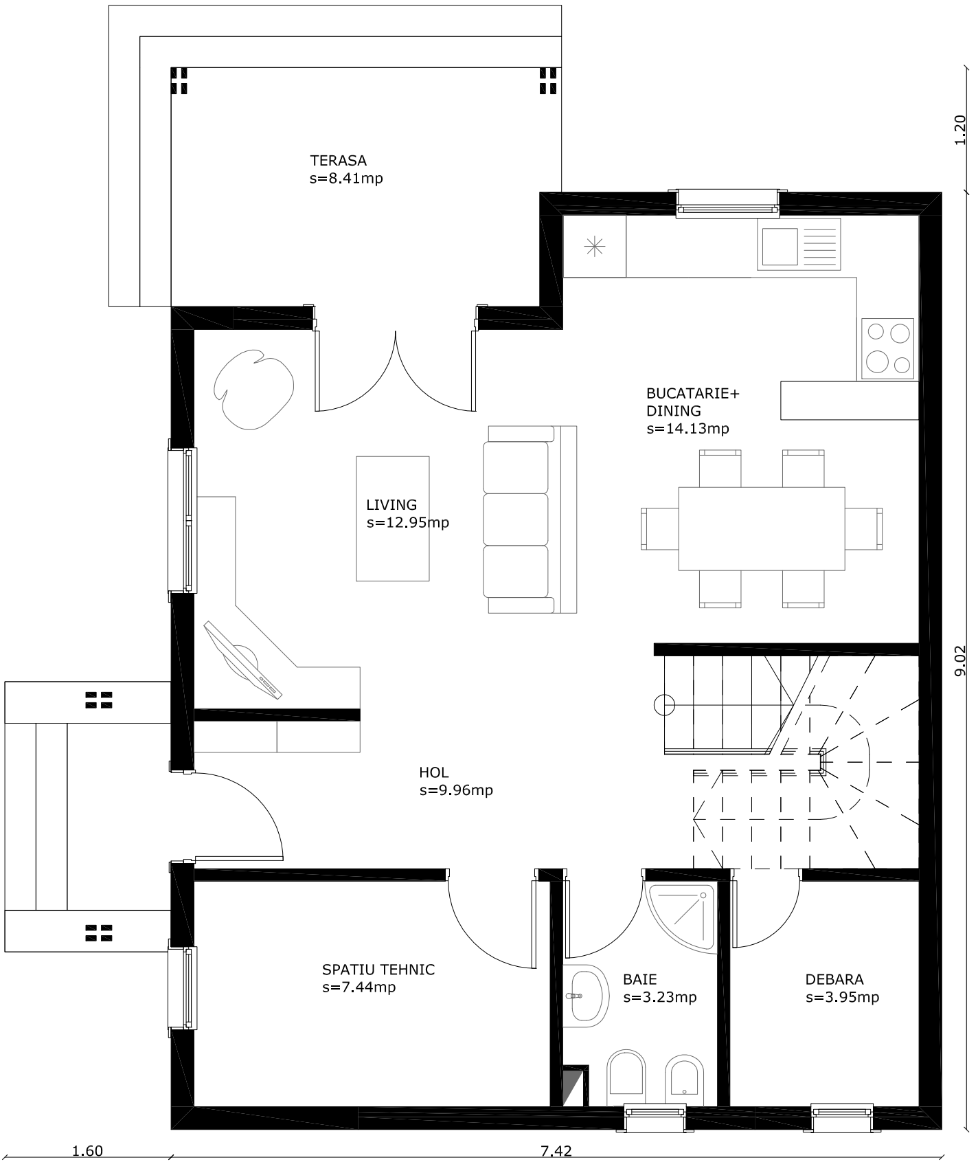
PLAN PARTER
